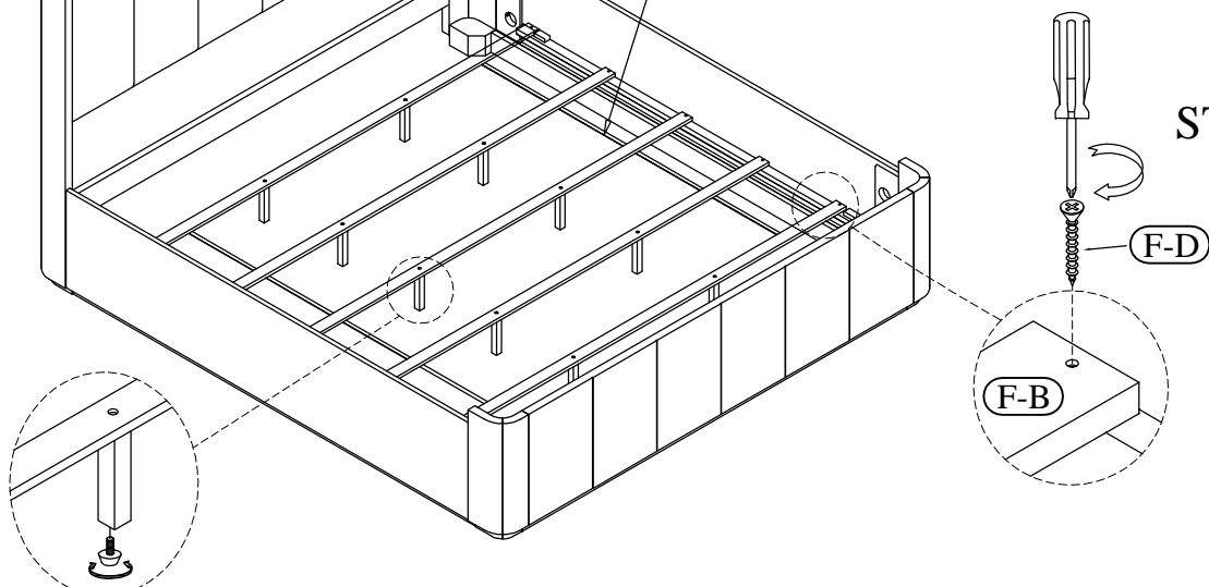
Adjustable Leveler
